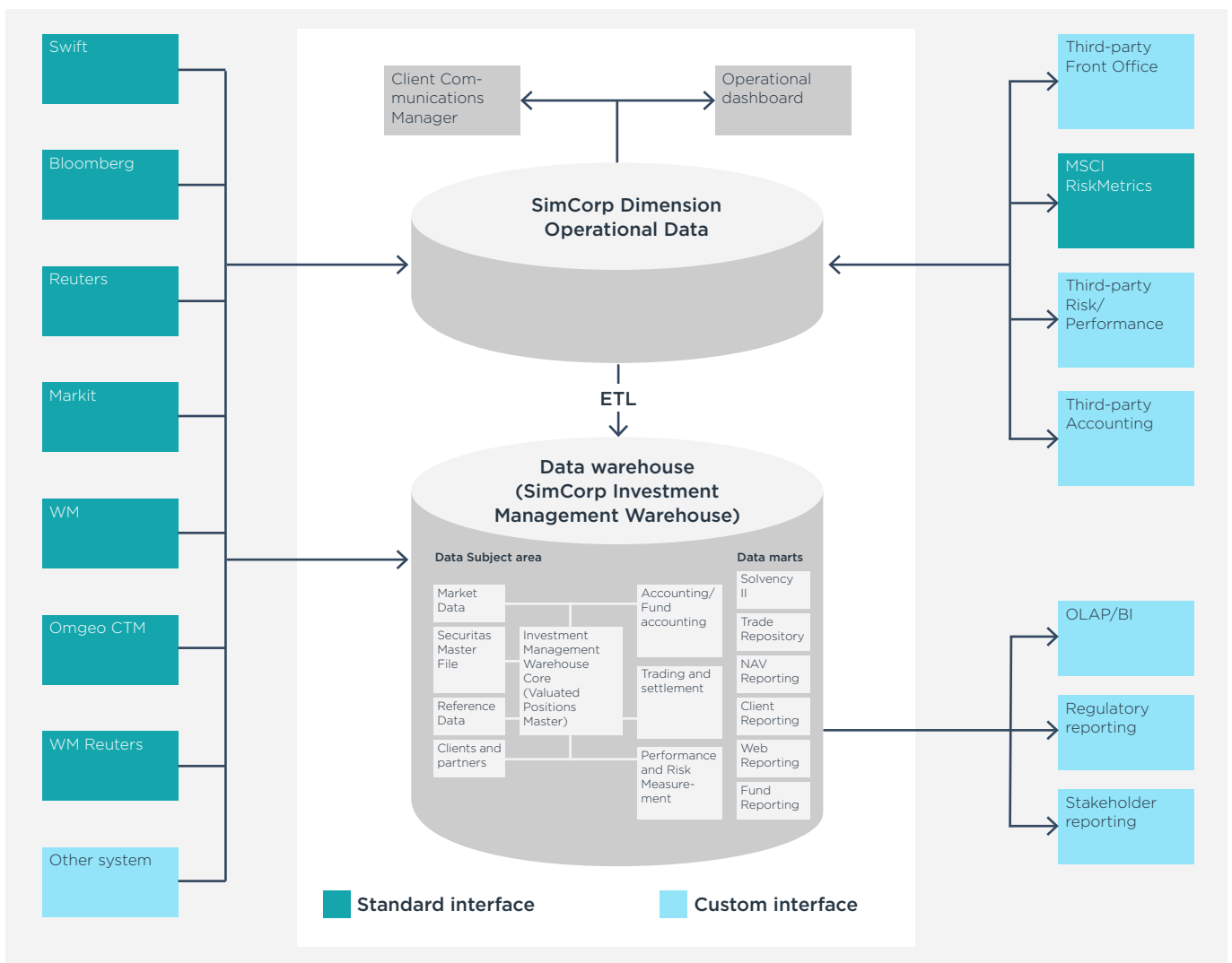
Process flow in Data Warehouse Manager. Data from anywhere in the front, middle, and back office is extracted into the SimCorp Dimension online transaction processing (OLTP) database. Along with market data and data from third-party applications, the OLTP data is included in the consolidation and quality-check workflows before the data goes into the data warehouse (SimCorp’s Investment Management Warehouse). The data is then ready for reporting and analytical queries.
